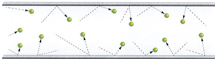
MOLECULAR FLOW - RANDOM MOVEMENT
